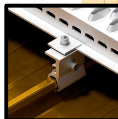
Support connection to roof bracket (Perpendicular - Angled)
