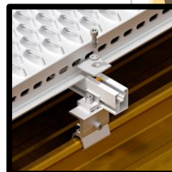
Support connection to roof bracket (Perpendicular - Flush)
