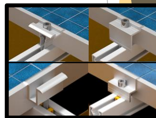
Clamp connection
