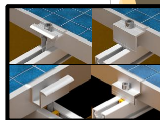
Clamp connection
