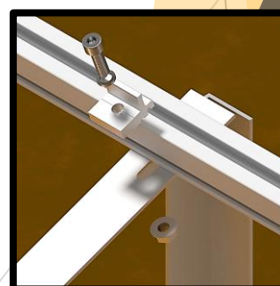
Rail connection to incline channel
