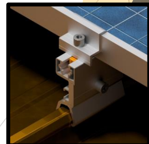
Clamp connection to roof bracket
