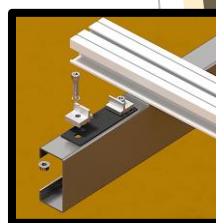
PV module position on Rails
