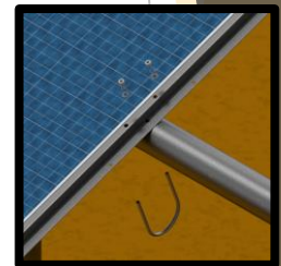
Post connection to Purlin
