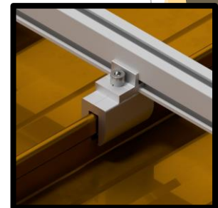
Integration with Railed system connection on standing rib
