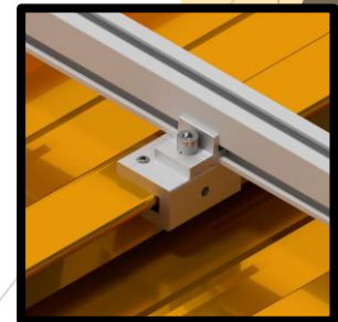
Integration with Railed system connection on horizontal rib
