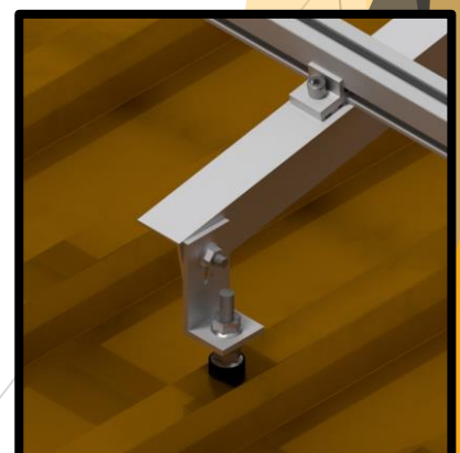
Integration with angled frame railed
