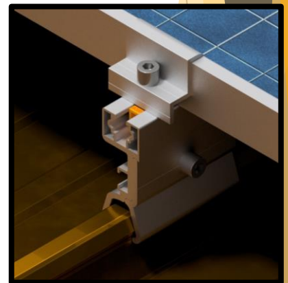
Integration with PV module connection
